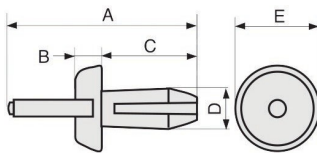
DUCTAFIX R6 Fixing rivet
