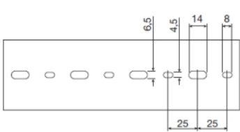
T1-ZH Widths 25, 40 and 60 mm Perforations in base
