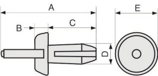
DUCTAFIX R4 Fixing rivet
