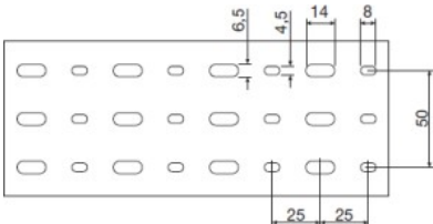
T1-ZH Widths 80, 100 and 120 mm Base holes
