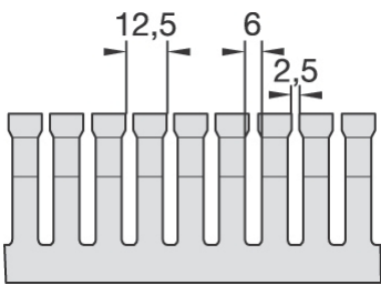
T1-ZH Pitch - Slot - Lamella
