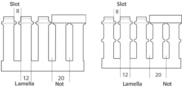
T1-N Depths 40 and 60 T1-N Depths 80 and 100
