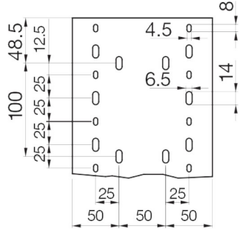
T1-N width 150 Perforated hole in base
