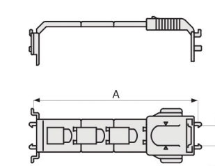
TR1N Wire retaining clip
