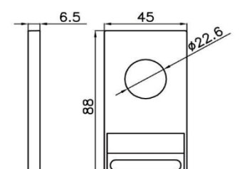
SCP Fixing element
