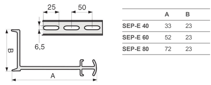
SEP-E Partition wall
