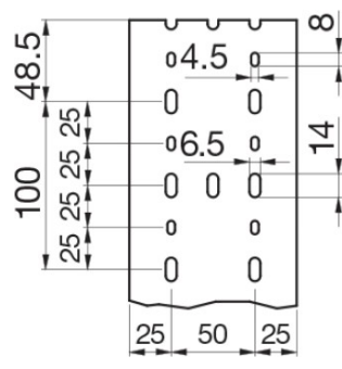
T1-N widths 80, 100 and 120 Perforated base
