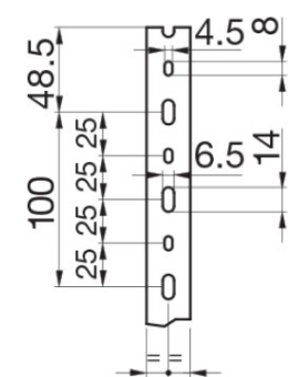
T1-N width 25 Base perforation
