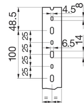
T1-N width 40 and 60 Perforated base
