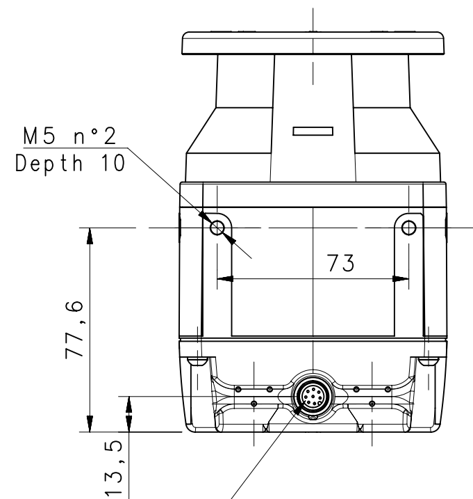
Male Connector M12x1 8-Poles A-Code
