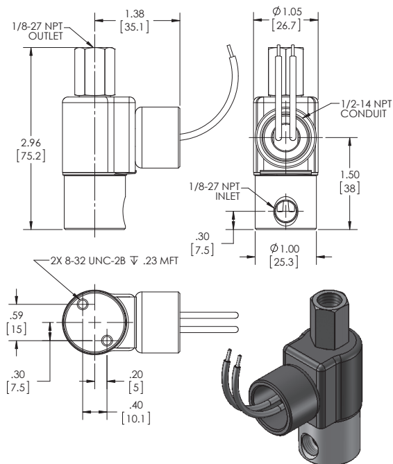
SERIES 50 MODEL 51 2WNO CONDUIT CONNECTION
