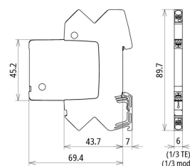
Dimension drawing BCO ML2 BD 12
