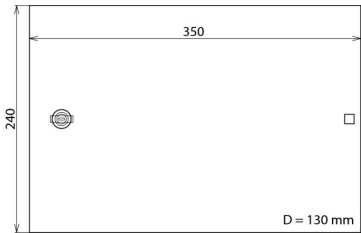
Dimension drawing DPG LSA 60 P
