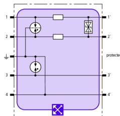
Basic circuit diagram BXT ML2 BD HFS
