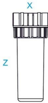
Single Filter 5" - X:130mm - Z:195mm 10" - X:130mm - Z:320mm Double Filter 5" - X:273mm - Z:195mm 10" - X:273mm - Z:320mm Triple Filter 5" - X:416mm - Z:195mm 10" - X:416mm - Z:320mm
