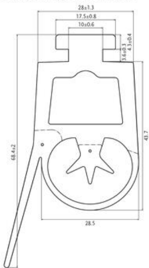
Profile cross-section Contact-Duo 3100.0804B
