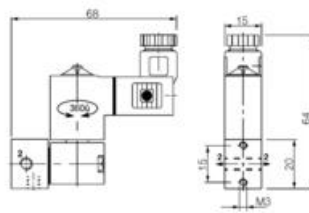
M5-connection
