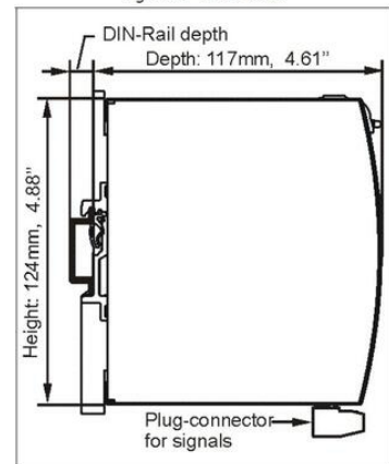
Fig. 24-1 Side view
