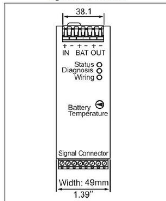
Fig. 25-2 Front view
