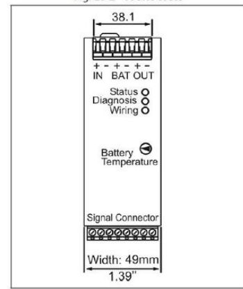
Fig. 25-2 Front view
