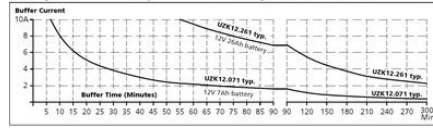
Fig. 9-1 Buffer time vs. output current with the battery modules UZX12.071 and UZX12.261
