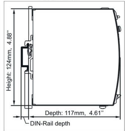
Fig. 20-2 Side view
